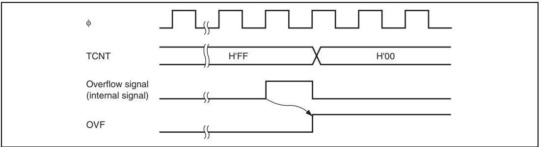
Figure 11.4 OVF Flag Set Timing
